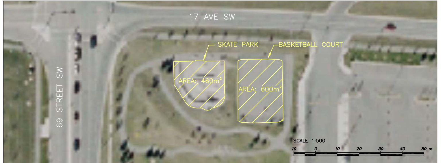
DETAIL A – EXISTING LOCATION OF RECREATION FACILITY
